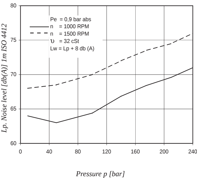
NOISE LEVEL (TYPICAL) - T7DCC - B31 - 022 - 022
