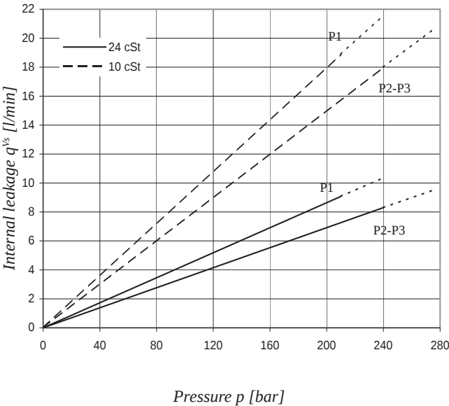
INTERNAL LEAKAGE (TYPICAL)
