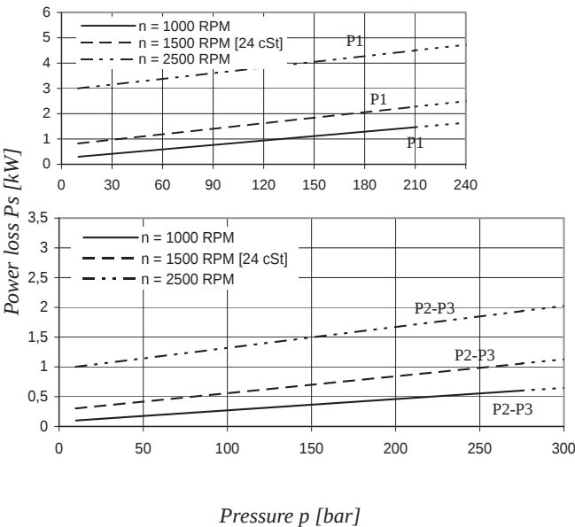
POWER LOSS HYDROMECHANICAL (TYPICAL)
